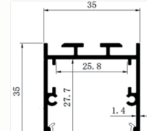
ML-035 3m Deep Surface Profile
