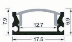
ML-071/081 2m Slim Surface Profile
