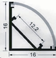
ML-106 2m Slim Corner Profile
